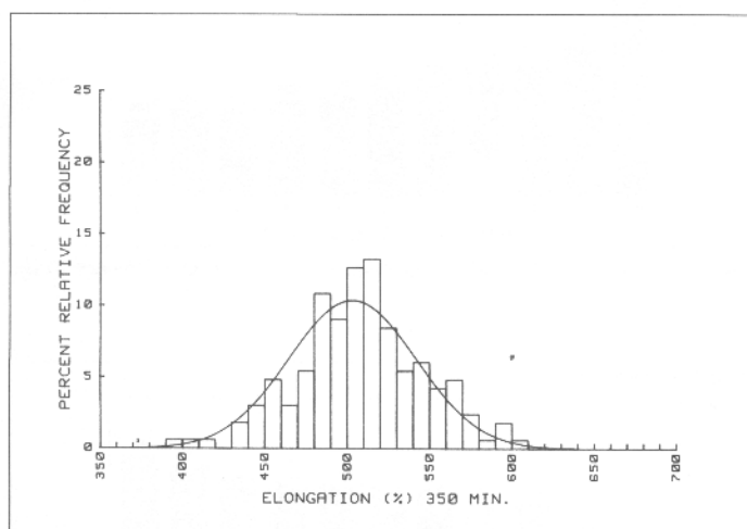
Figure 19 EPDM (465), fourth quarter 1983.
