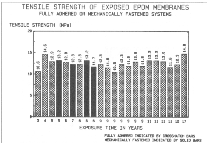
Figure 1 Tensile strength of exposed EPDM membranes—fully-adhered or mechanically-fastened systems.
