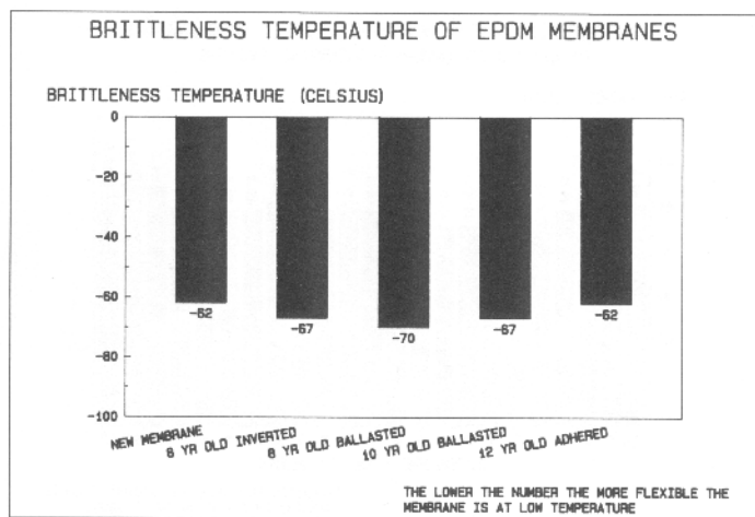
Figure 9 Brittleness temperature of EPDM membranes.
