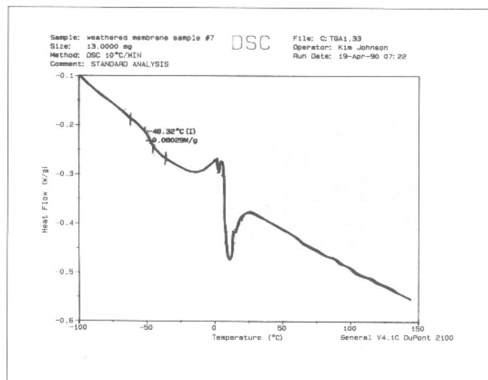
Figure 11 DSC—weathered membrane sample #7.
