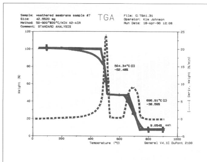
Figure 10 TGA—weathered membrane sample #7.
