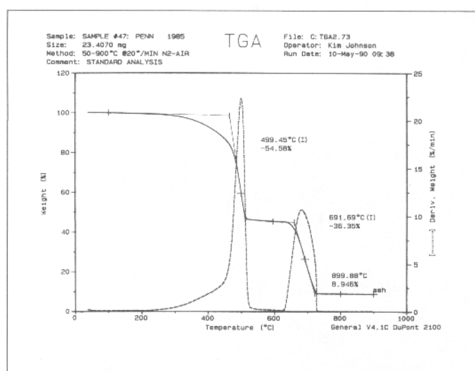
Figure 22 TGA—sample #47, Pennsylvania 1985.
