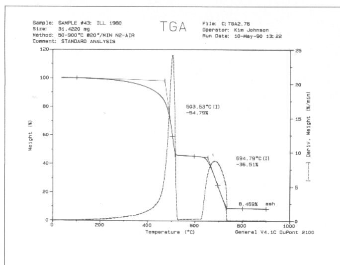
Figure 23 TGA—sample #43, Illinois 1980.
