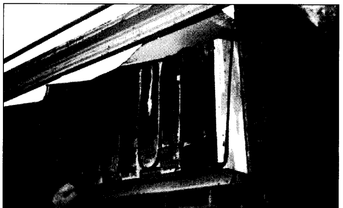
Figure 11. Heater laid in channels routed in the plywood sheathing behind the fascia metal.
