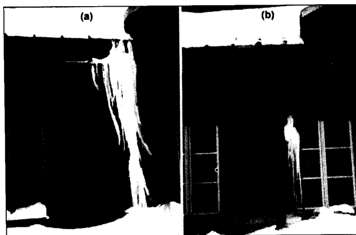
Figure 9. (a) Large icicle created by a high-powered valley heater and (b) three days later, its remnant hanging from the displaced, but still operating heater.
