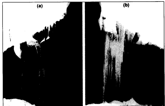
Figure 14. Comparison of heated and unheated valleys at Building 10210 on February 22, 1993: (a) Heated valley and heated false fascia clear of ice. (b) Adjacent unheated valley and fascia encased in ice.
