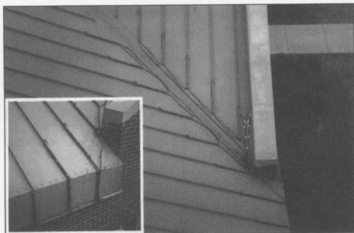
Figure 4. System with multiple heater runs in the valley, behind the parapet and on several standing seams. Inset shows heater runs at its fascia and drip edge.
