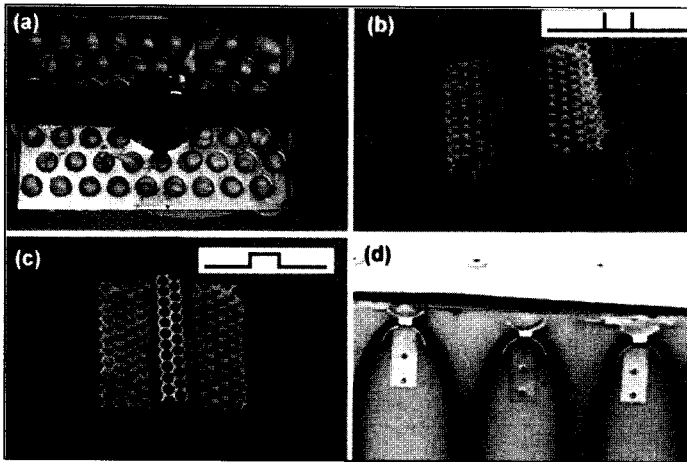
Figure 10. Heater attachments adhered with high strength neutral-curing silicone are: (a) dome, (b) channel, and (c) tunnel clips. The commercially available butterfly clip (d) was mechanically attached with rivets or screws.
