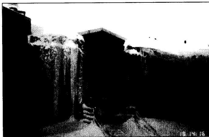
Figure 1. Severe, problematic icings and ice dams along eaves of a dining facility at Fort Drum in upstate New York.
