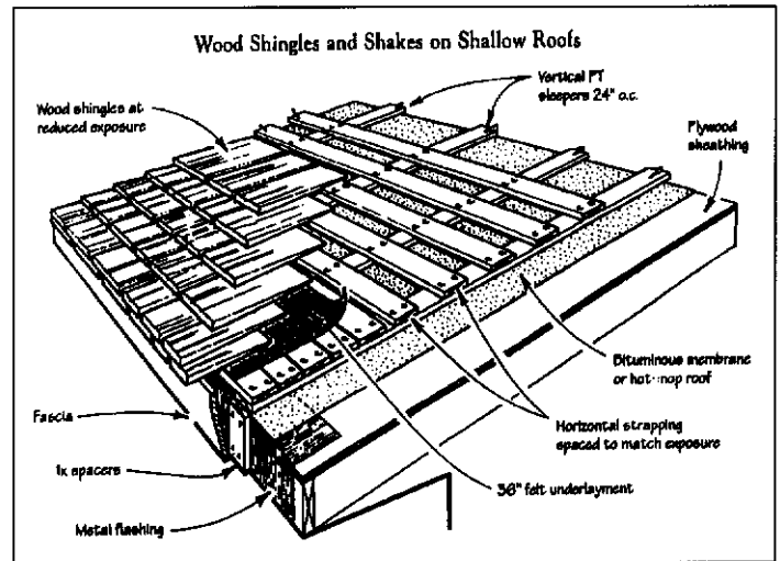
Figure 3. On shallow slopes, install wood shingles and shakes over a watertight subroof and a framework of pressure-treated strapping. The fascia is spaced out from the metal flashing at the eaves to allow any water that gets under the roofing to drain from the subroof. From Wardell [17].
