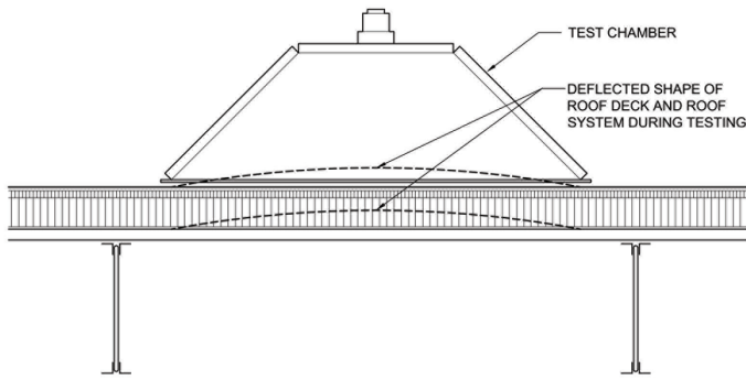
Figure 1: Illustration of a test chamber positioned between deck supports
