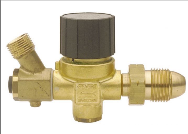
Photo 7: Preset-type pressure regulator.
