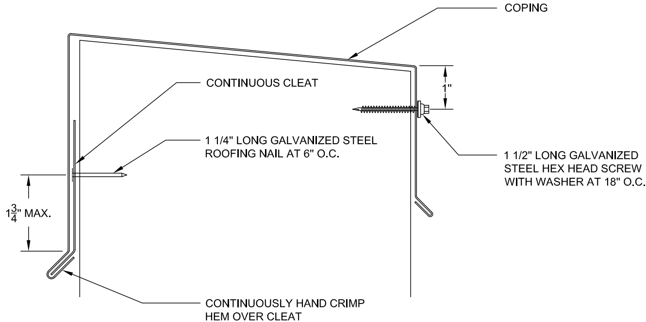
INSTALLATION
