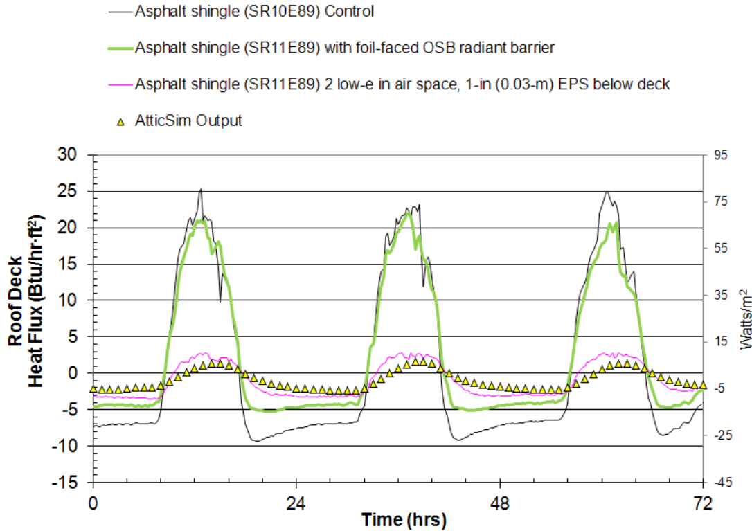
Figure 5 Heat flux crossing the roof deck of the asphalt shingle roofs for three consecutive winter days in the climate of East TN. Average daytime and nighttime temperatures (48/38) ° F. Field data for February 2010 is benchmarked against AtticSim (triangle symbols are AtticSim prediction)
