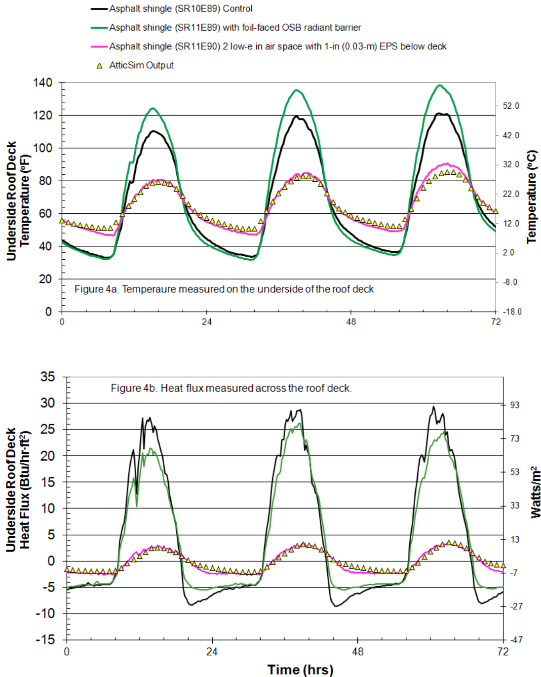
Figure 4 Temperature measured on the underside of the roof deck (4a) and the measured heat flux crossing the roof deck (4b). Field data for August 2010 is benchmarked against AtticSim (triangle symbols are AtticSim prediction)
