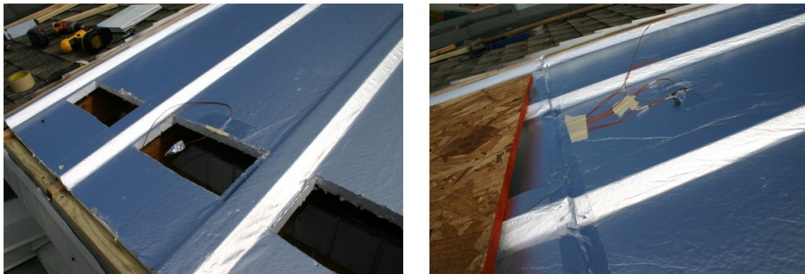
Figure 3. Setup of a prototype roof for new construction shows the EPS with vent slots and a perforated foil-faced OSB deck lying on top of the EPS to create an air space. The slots in EPS provide a passageway for air from the soffit vents and also from the attic space.
